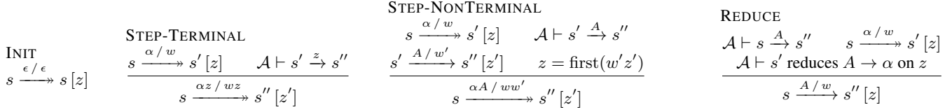
Figure 4. Inductive characterization of the “fact” and “edge fact” predicates.
